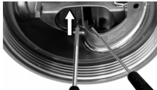
Fig. 16 – Retaining Ring Removal
