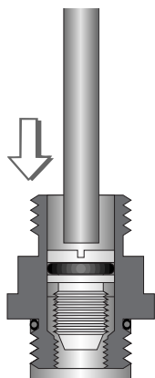
Fig. 24 – Orifice Installation
